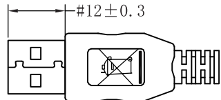
CONN. 2 USB A TYPE MALE
